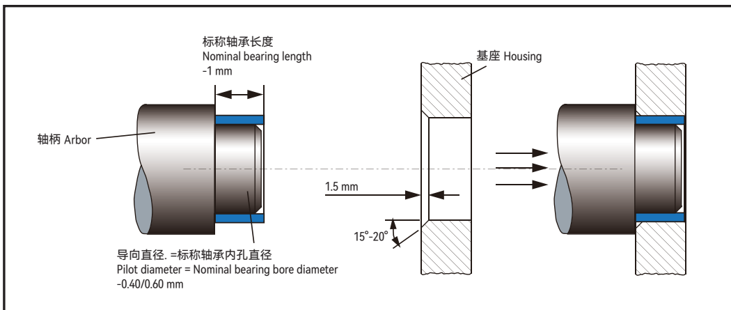
轴承的安装 Bearing Installation
